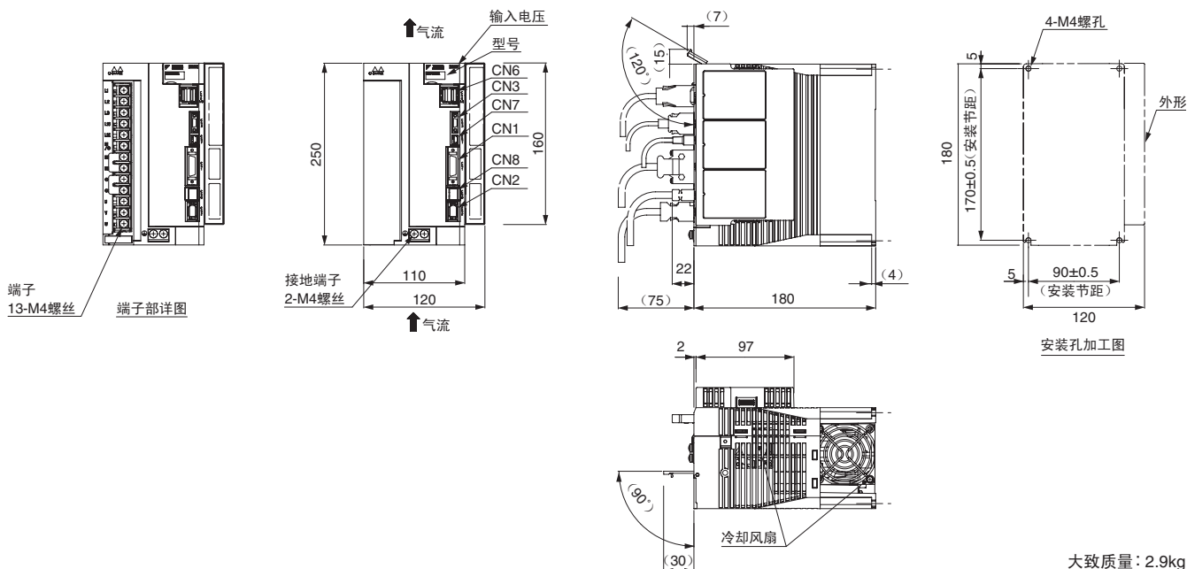
(7) 三相 AC200V SGD180A1□A000000001、SGDV200A1□A000000001
