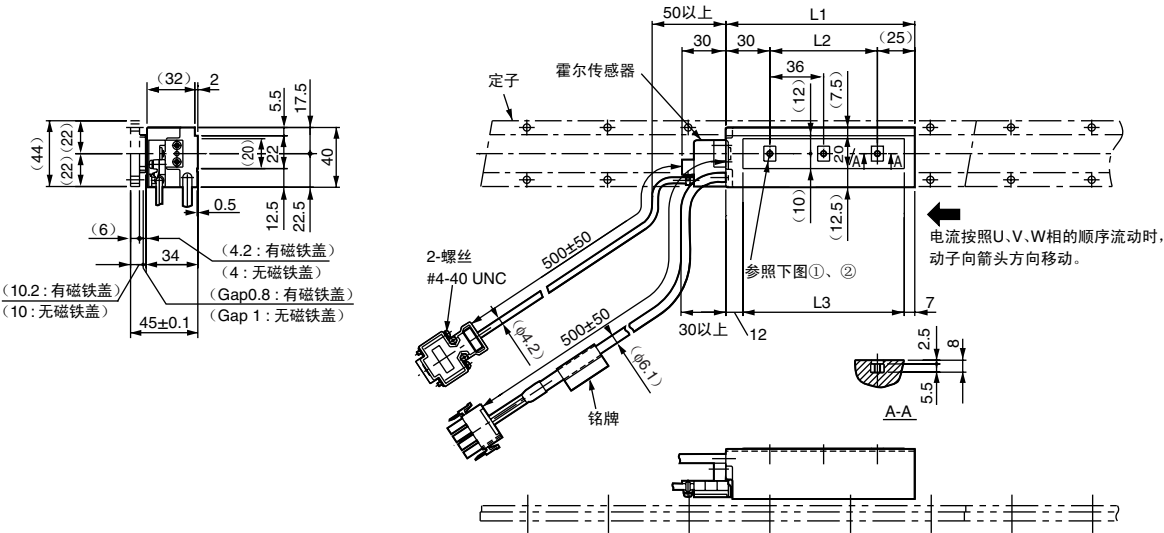
①SGLFW-20A090A□
