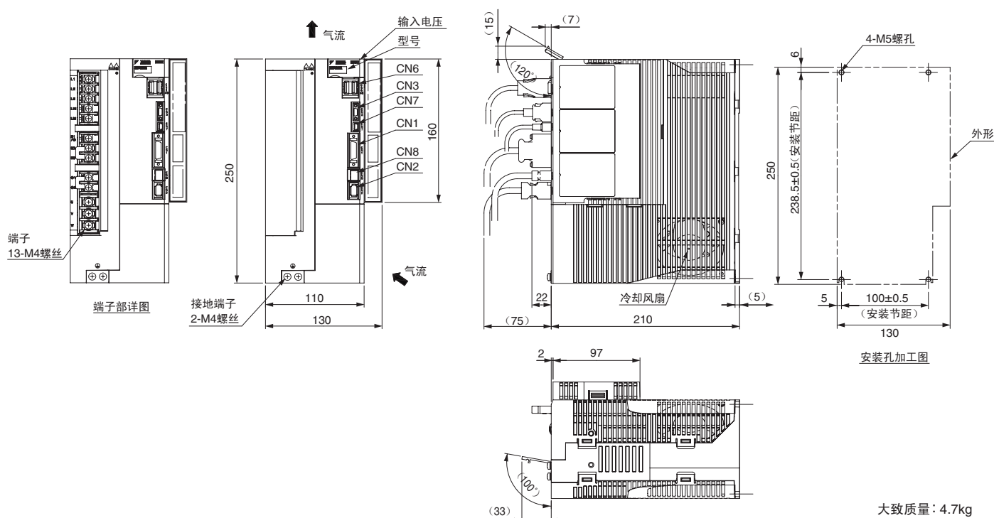
(8) 三相 AC200V SGD330A1□A000000001
