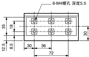
①SGLFW-35□120A□D
