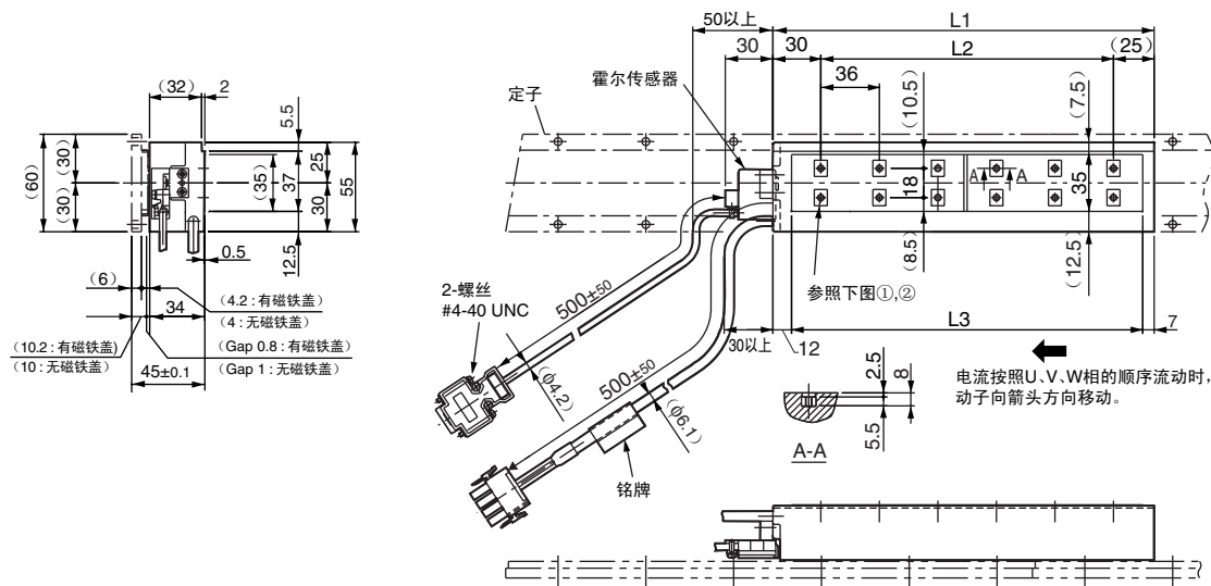
① SGLFW-35□120A□
