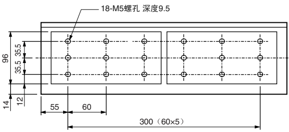
②SGLFW-1ZD380B□B
