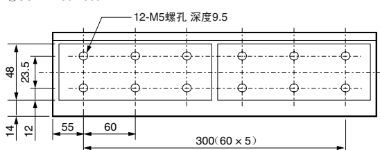
② SGLFW-50□380B□D
