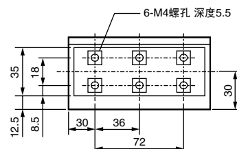
① SGLFW-35□120A□
