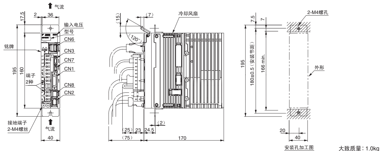
(5) 三相 AC200V SGD V-3R8A1□A001、-5R5A1□A001、-7R6A1□A001
