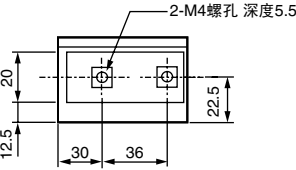
①SGLFW-20A090A□
